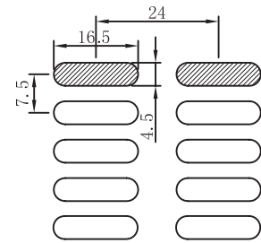
No. P29a | Max. width 300mm Thickness 0.87mm Open Area 38.8%
