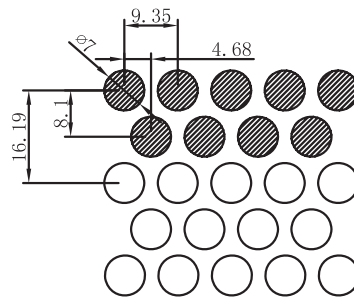
No. P35 | Max. width 710.6mm Thickness 0.7~0.8mm Open Area 50.8%
