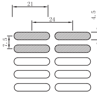
No. P29 | Max. width 1053mm Thickness 0.7mm Open Area 50%
