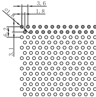
No. P20 | Max. width 702mm Thickness 0.5mm Open Area 22.8%
