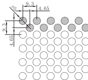
No. P25 | Max. width 576.6mm Thickness 0.5-0.7mm Open Area 45.38%
