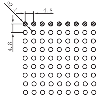
No. P38 | Max. width 864mm Thickness 0.7~0.8mm Open Area 19.6%
