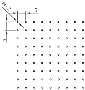
No. P28 | Max. width 750mm Thickness 0.5mm Open Area 2.0%
