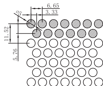
No. P33 | Max. width 705mm Thickness 0.7-0.8mm Open Area 51.3%
