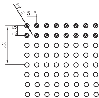
No. P39 | Max. width 1138.5mm Thickness 0.5~1.0mm Open Area 16.2%
