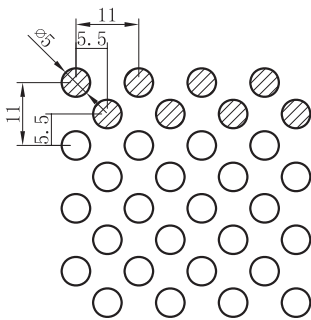
No. P45 | Max. width 275mm Thickness 0.7mm Open Area 30%
