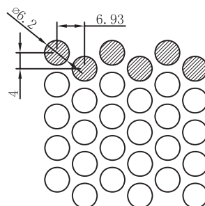
No. P32 | Max. width 714mm Thickness 0.7-0.8mm Open Area 54.44%
