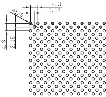
No. P17 | Max. width 705.2mm Thickness 0.5mm Open Area 19.1%
