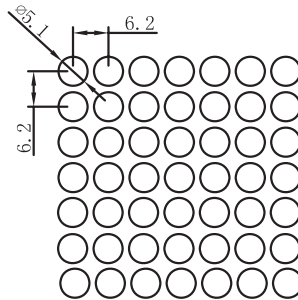
No. P41 | Max. width 624mm Thickness 0.5~0.8mm Open Area 46.5%
