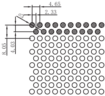
No. P34 | Max. width 706.8mm Thickness 0.7~0.8mm Open Area 37.8%
