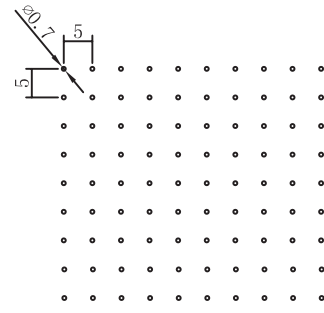
No. P21 | Max. width 690mm Thickness 0.5mm Open Area 1.54%
