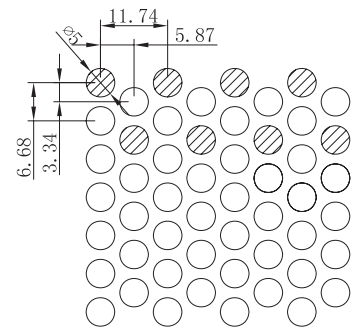
No. P47 | Max. width 821.8mm Thickness 0.7mm Open Area 45.6%
