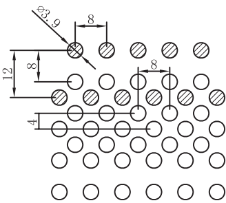
No. P22 | Max. width 712mm Thickness 0.7mm Open Area 37.3%
