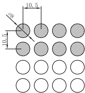
No. P31 | Max. width 1050mm Thickness 0.5-0.8mm Open Area 45.6%
